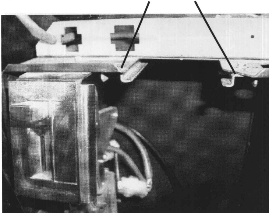
Figure 1 Bill transport removed / view of track for bill transport
